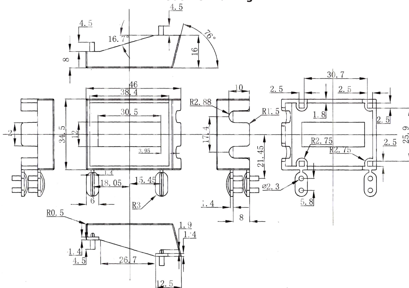
Outline Drawing
